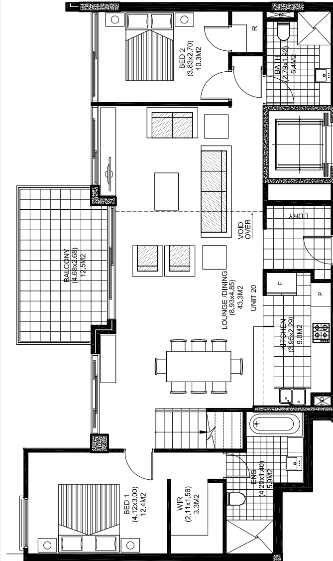
FLOOR LEVEL 3
